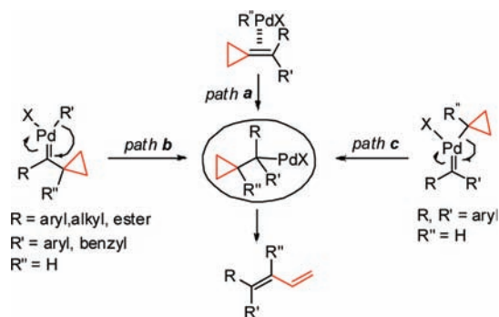
Scheme 1. Routes to the Cyclopropylmethyl Palladium Species
