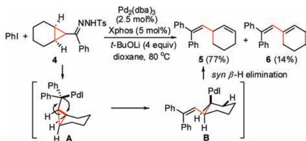
Scheme 2. Cross-Coupling of Iodobenzene with 4
